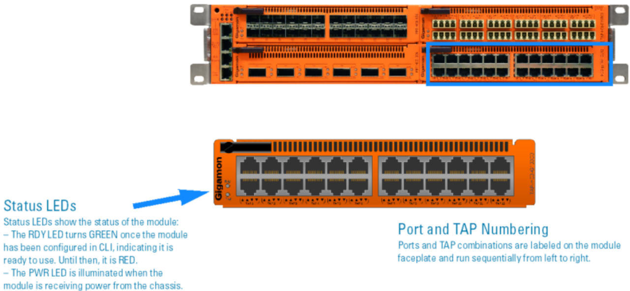
Figure 12 TAP-HC0-G100C0 Module
