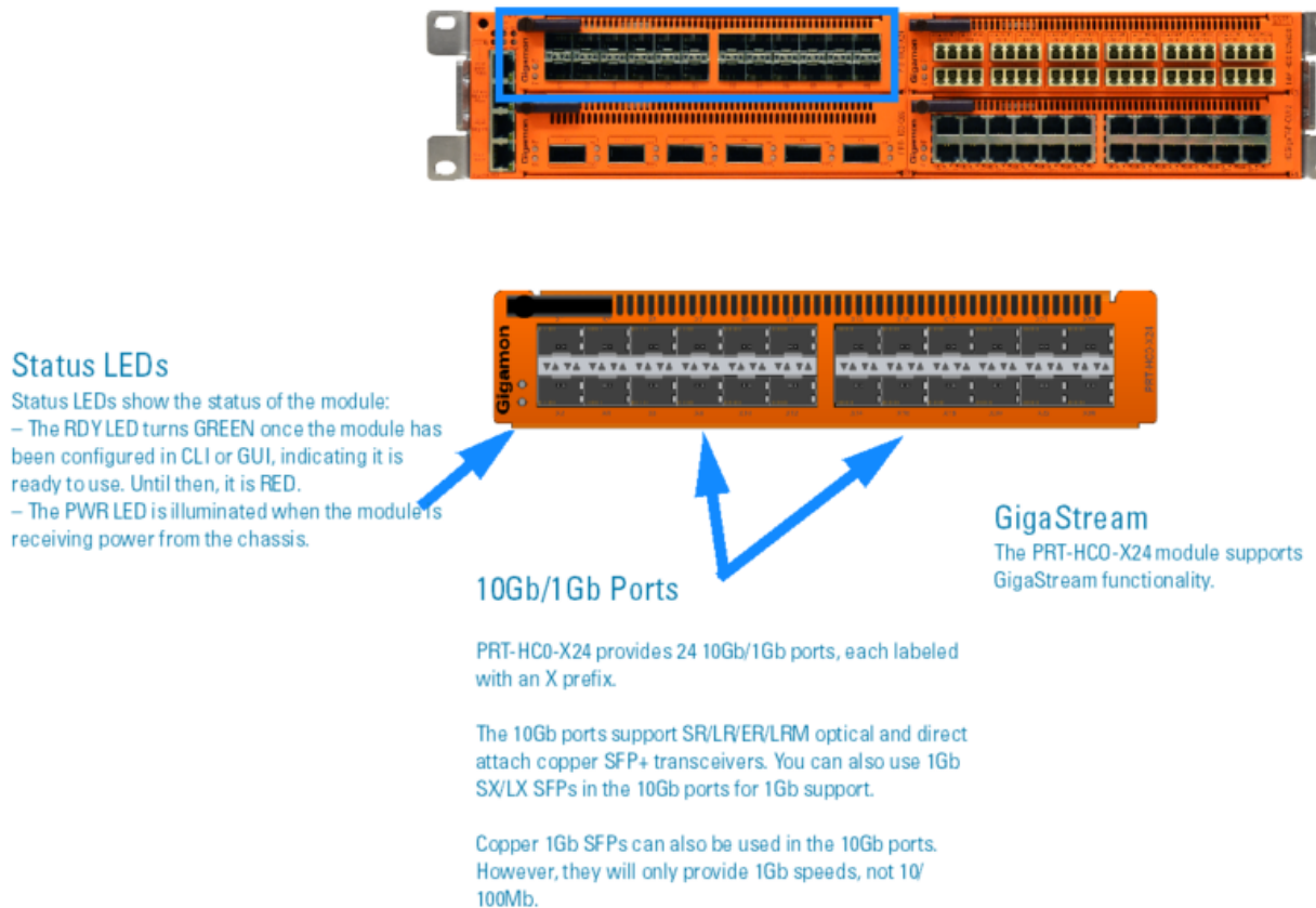
Figure 4 PRT-HC0-X24 Module
