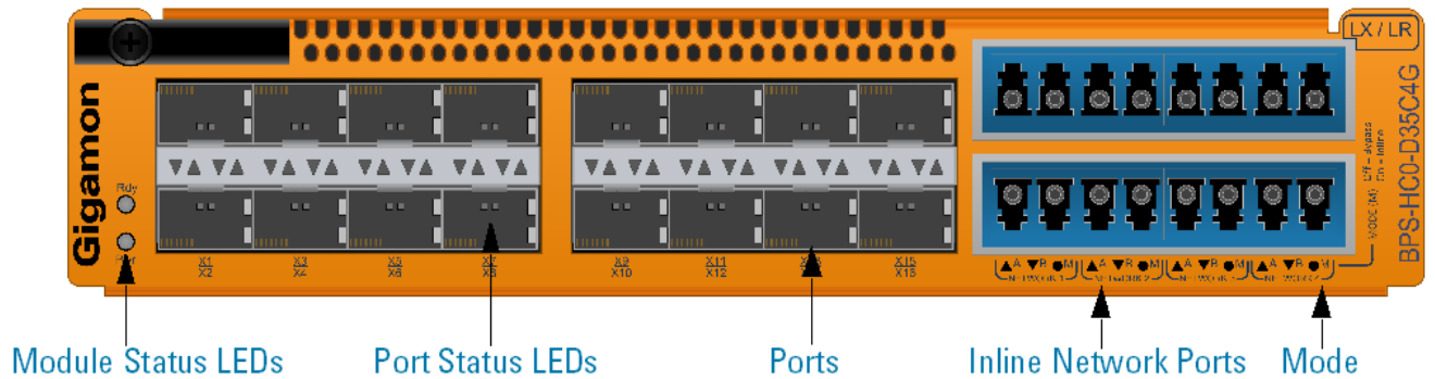
Figure 15 Bypass Combo Module BPS-HC0-D35C4G
