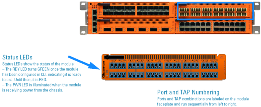
Figure 11 TAP-HC0-D35CC0 Module
